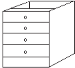
4 DRAWER CHEST 980 High 4 x 215 Drawers
